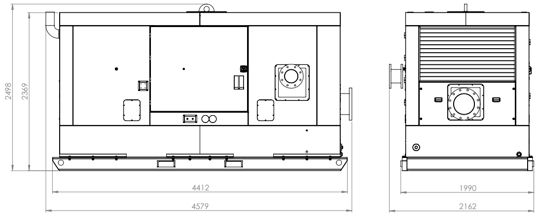
Weight (Dry / Wet): 6900 kg / 7500 kg
